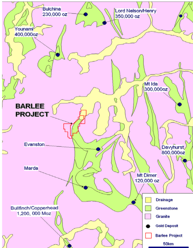
Barlee Project – Regional Location Map
