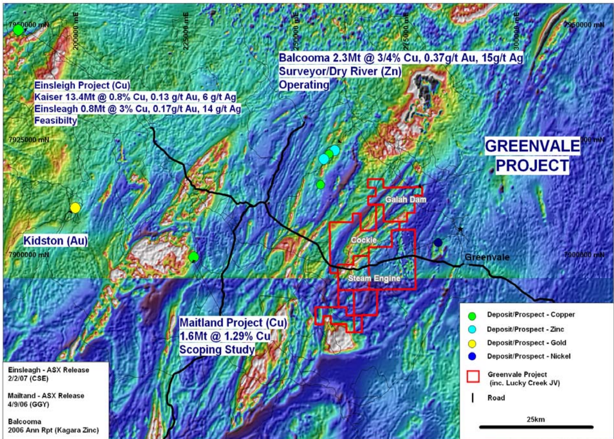
Greenvale Project – Location Map overlain on regional magnetics
