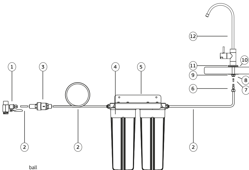
Figure 1 - Parts Diagram
