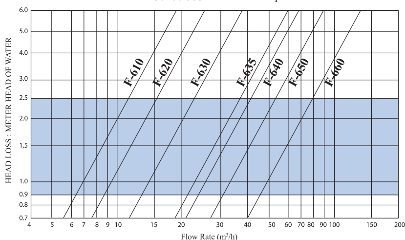
Series 600 - Head Loss Graph
