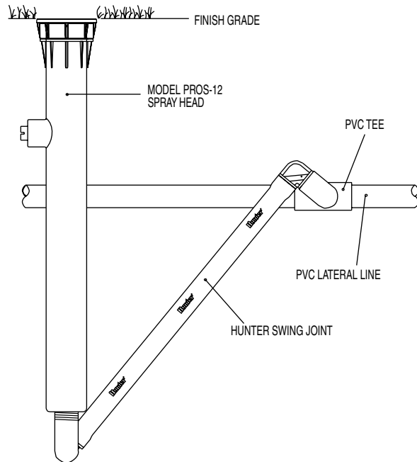
Hunter® PROS-12
